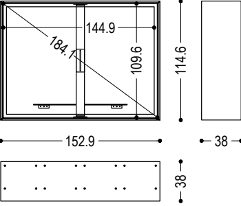
FREEDOM-TV 2-REV (REVOLVING BACK)
