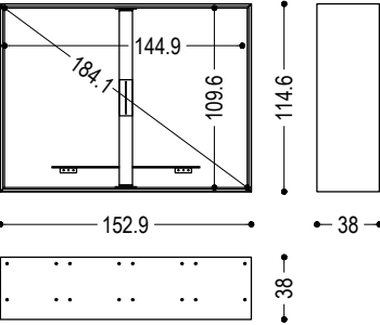
FREEDOM-TV 2 (FIXED BACK)
