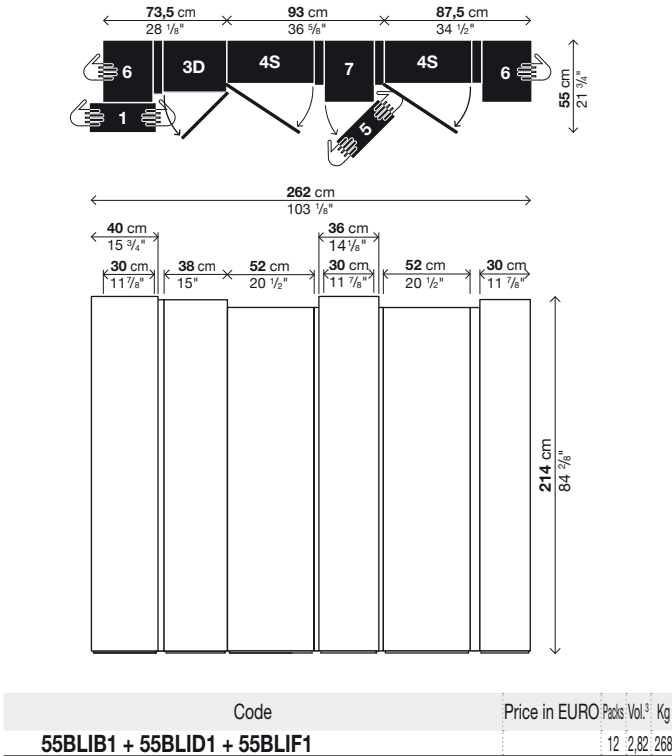
Composition B8 Unit B + Unit D + Unit F
