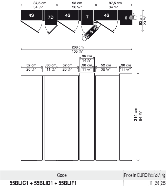
Composition B7 Unit C + Unit D + Unit F
