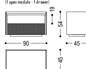
REVO NIGHT TABLE 2.2 (1 open module - 1 drawer)
