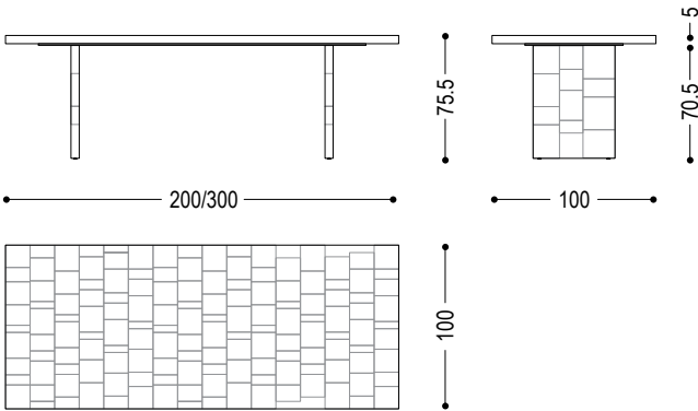
Drawing of top and base for illustrative purposes only
