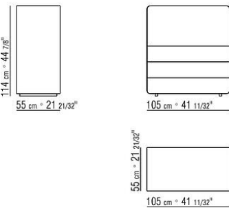
COD. 02F775 CABINET
