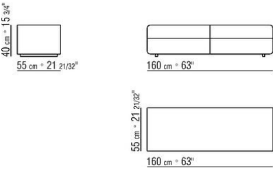
COD. 02F777 CABINET
