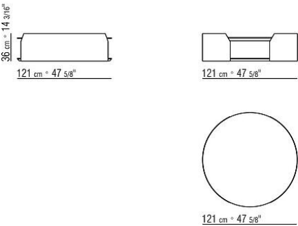
COD. 02G172 COFFEE TABLE
