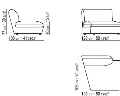
COD. 02F461 END UNIT SLANTED L
