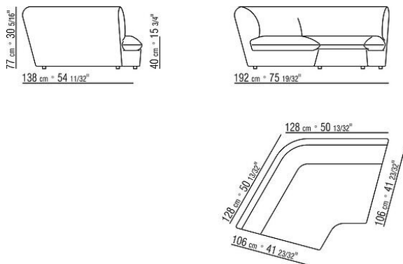
COD. 02F432 CORNER SLANTED
