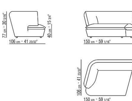
COD. 02F461 END UNIT SLANTED L
