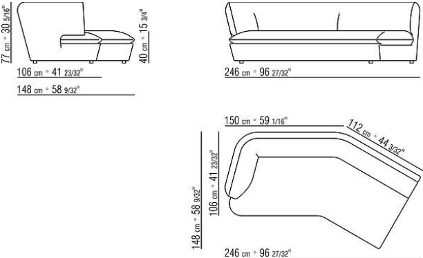
COD. 02F473 SIX SIDED END UNIT L
