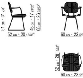
COD. 028007 S.H.-CHAIR W/ARMRESTS
